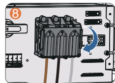
8 Close the box cover
