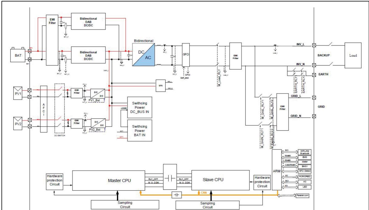
Design schematic diagram of inverter (GW3600-SBP-20, GW5000-SBP-20) as follows:
