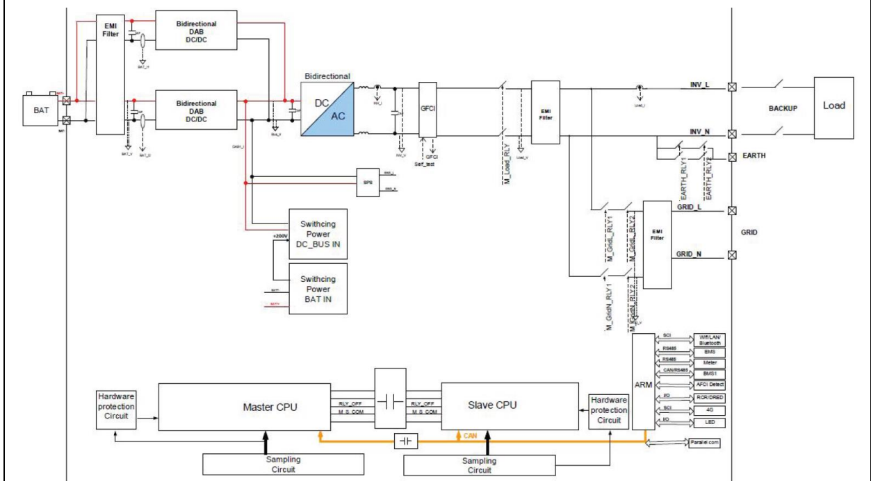
Design schematic diagram of inverter (GW3600-SBP-20, GW5000-SBP-20) as follows:
