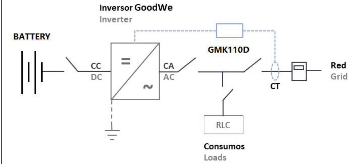
Battery-Grid mode of inverter GW3600-SBP-20, GW5000-SBP-20:
