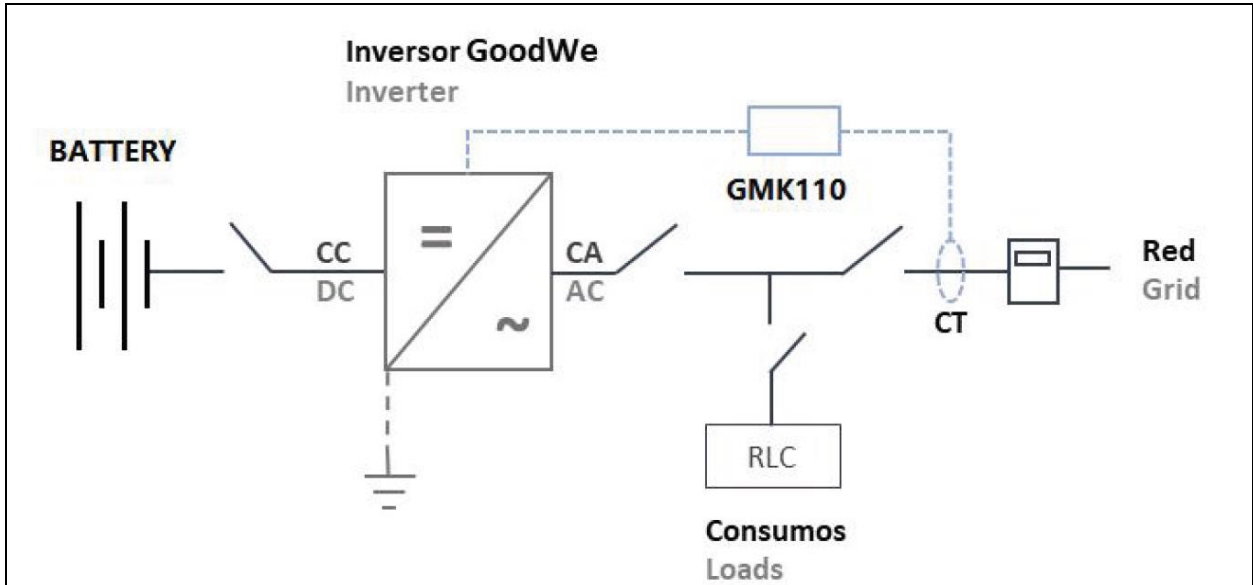
Battery-Grid mode of inverter GW3600-SBP-20, GW5000-SBP-20:
