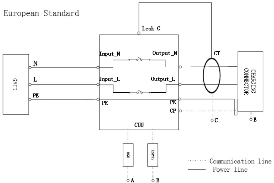
figure 3-1 Circuit diagram(European)
