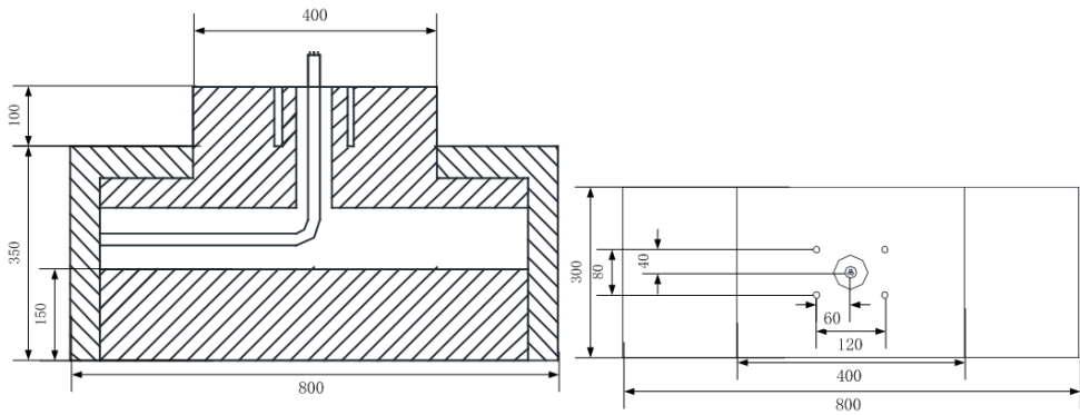
figure 3-7 Front view and top view (unit: mm)
