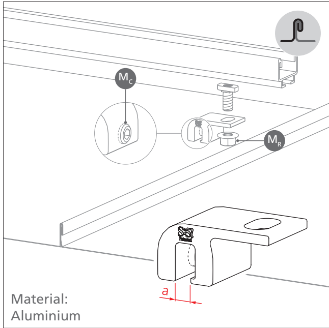
S-5! E-Mini-FL Standing Seam Clamp
