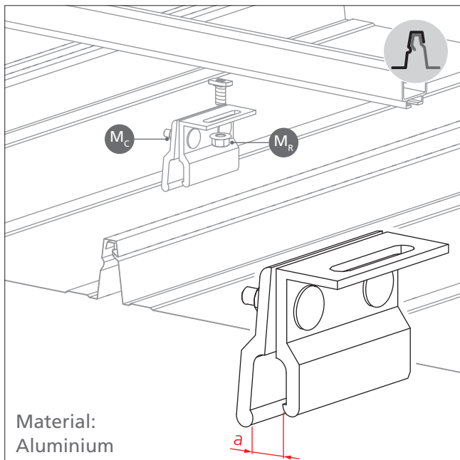
Rib-Roof Speed 500 Clamp
