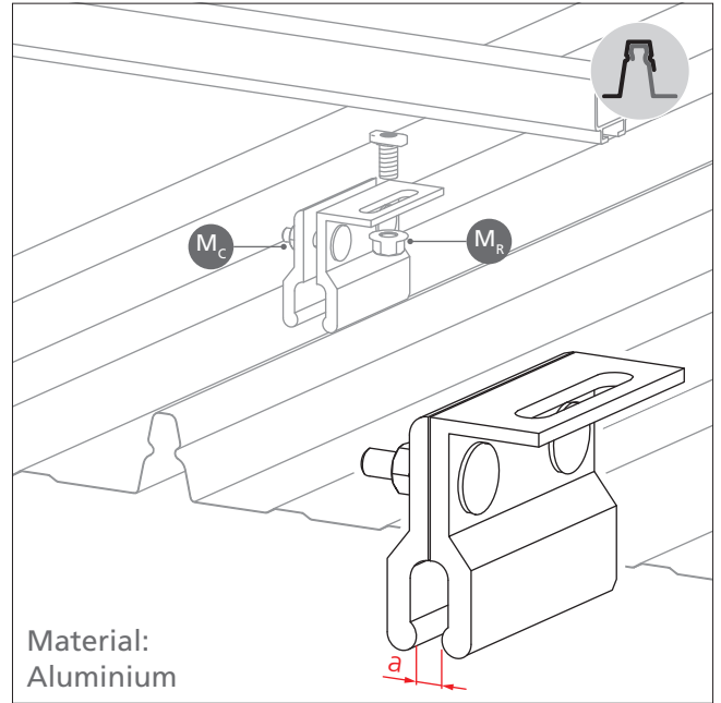
Rib-Roof 465 Clamp
