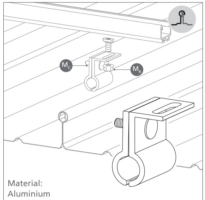
Rib-Roof Evolution Clamp
